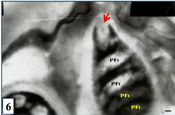
Figure 6. Transmission electron microscopy of longitudinal section through M. dermatobius parasite from the eye of Oreochromis niloticus , showing well developed polar capsule, four turns of polar filament (PFt) and apical cap (arrow). Scale bar = 500 nm.
