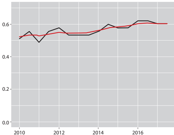
Figure 3. Percentage of countries reporting PTB presence from 2010 to 2017. Black line shows the real values and red line shows the trend. [Data from World Animal Health Information System (WAHIS)].
