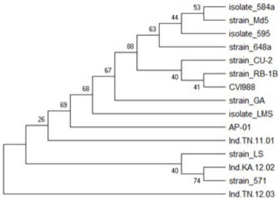
Figure 18. Phylogenetic analysis of Meq gene nucleotide sequence of AP-01 with other reference sequences. The phylogenetic tree was constructed using the MEGA version 10.0 by the neighbor joining method with 1,000 bootstrap replicates using Tamura nei model.
